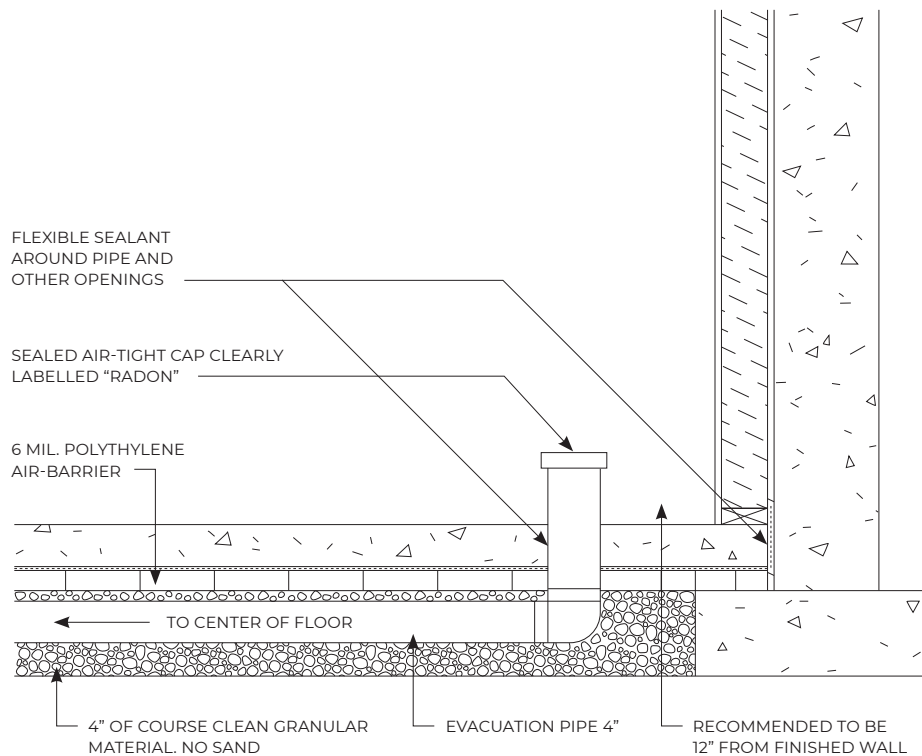
PENETRATION THROUGH SLAB DETAIL
